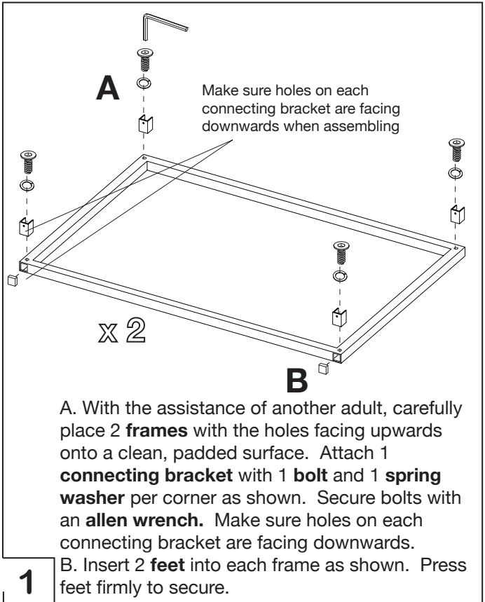
allen wrench (included)
