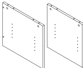
2 - side panels (1 left, 1 right)
